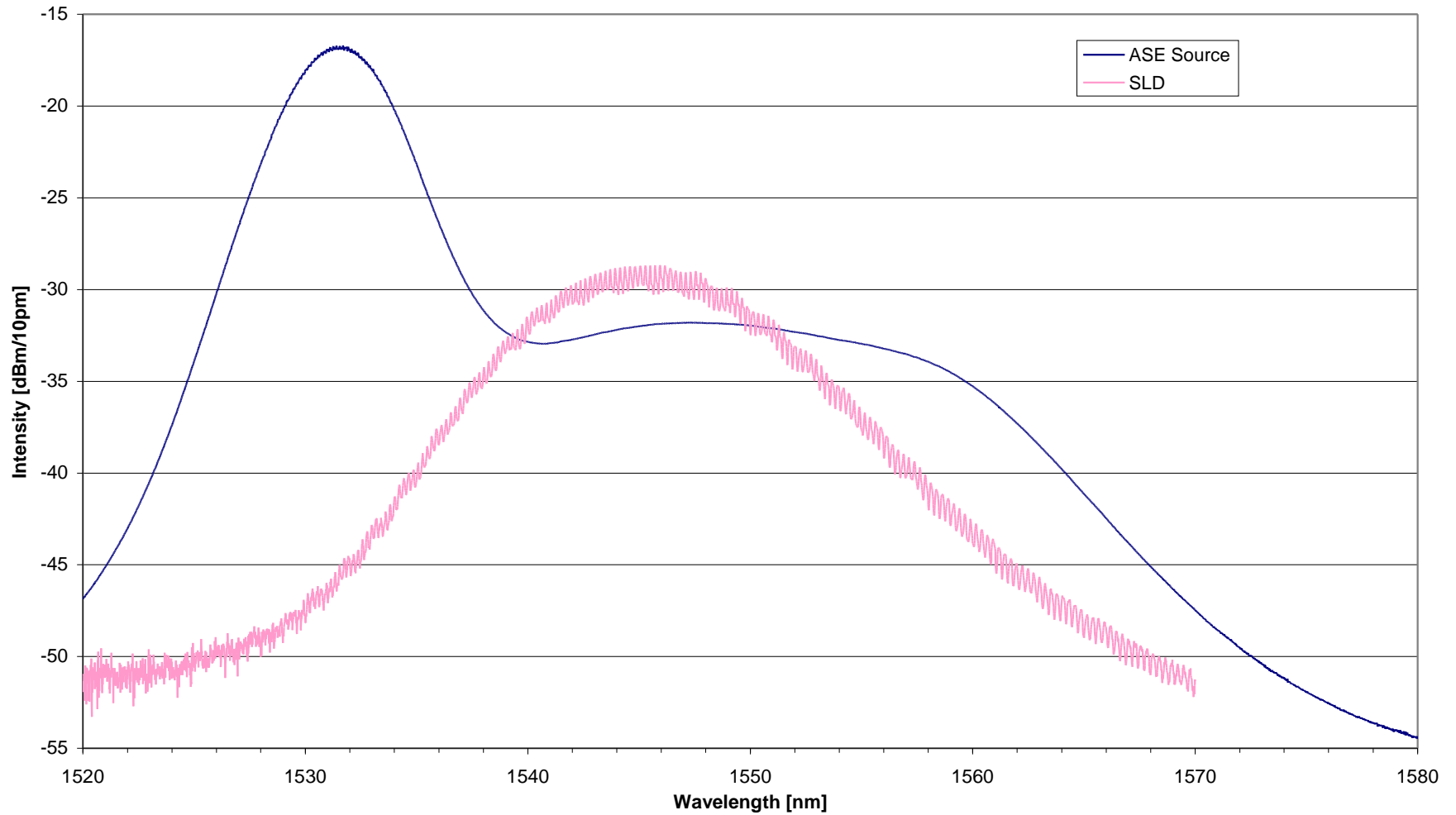
Spectra of a C-band ASE source and a superluminescent diode (SLD)
